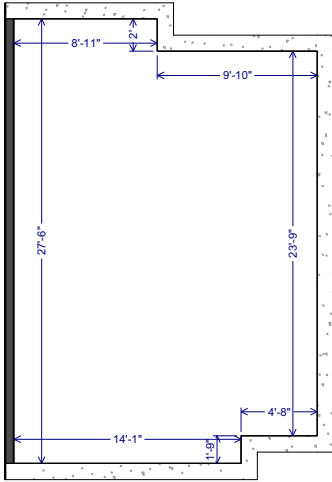
BASEMENT
